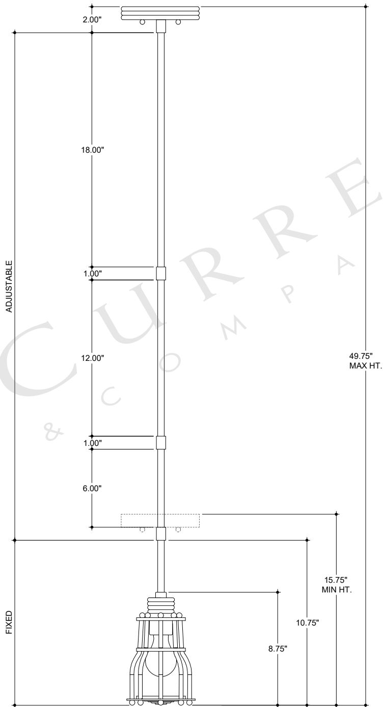
FRONT VIEW
